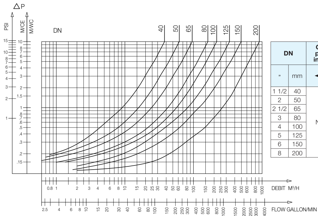
407 - Headloss chart
