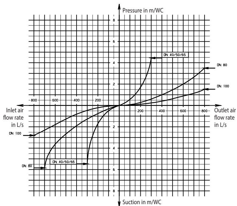
VE320 - Bend flow/pressure
