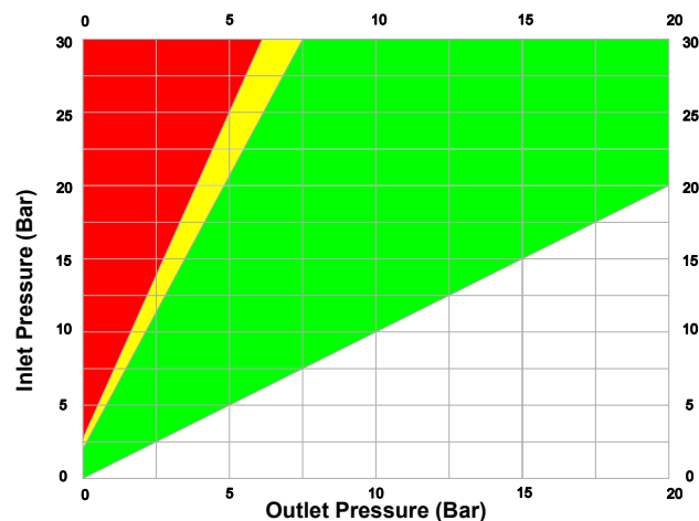
Cavitation chart of N200
