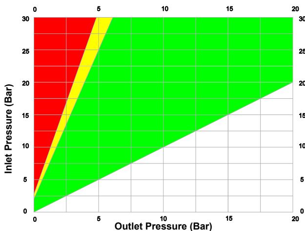
Cavitation chart of NR200
