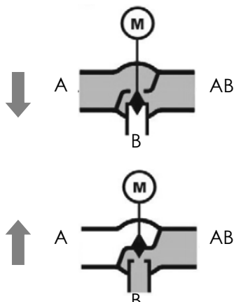
3-port Mixing Valve
